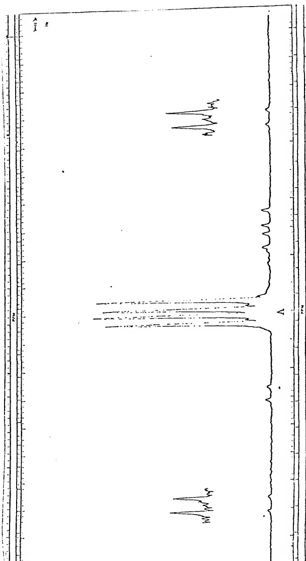
Figure 15 - ^{19}\text{F} NMR of \text{CF}_2\text{BrCFClCH}=\text{CHCl}_3 A
